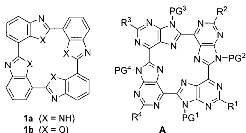
Figure 1. Quatercompounds 1 and general structure of tetrameric purines A .
