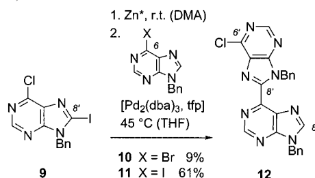
Scheme 4. Bond formation between C-6 and C-8' by Negishi cross-coupling.
