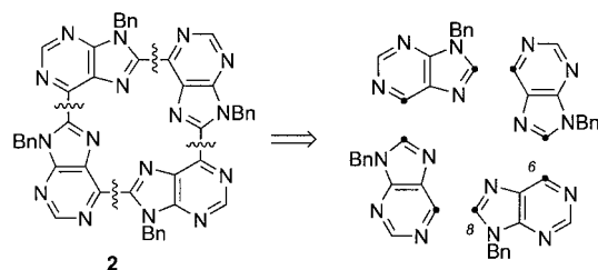
Scheme 1. Target compound 2 and disconnection into four purine units which need to be connected at the indicated (•) positions.
