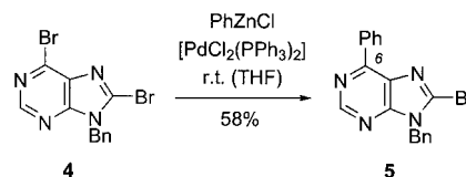
Scheme 3. Regioselective cross-coupling at position C-6 of dibromopurine 4 .
