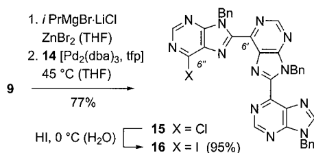
Scheme 5. Synthesis of the trimeric purines 15 and 16 .
