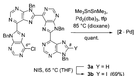
Scheme 6. Completion of the synthesis starting from the open tetrameric purine 3a .
