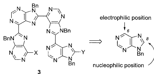
Scheme 2. Basic retrosynthetic consideration for the construction of open chain precursor 3 .
